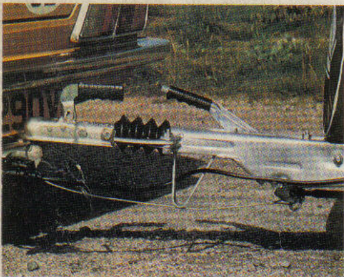
Inertia braking system recommended for use with small cars.
