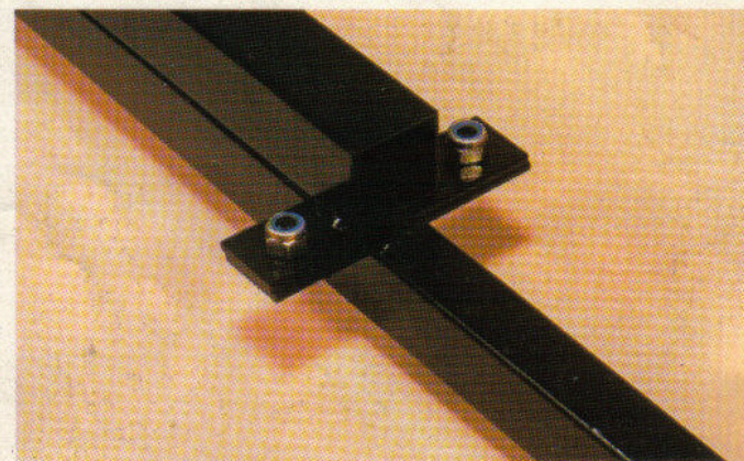
Removable trailer tow bar firmly secured with 4 self-locking nuts.
