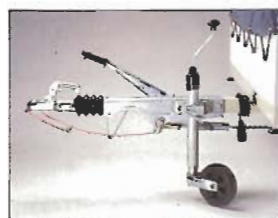
Brakes & Jockey Wheel
