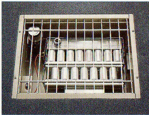
RIVIERA DE-LUX UNDER FLOOR HEATER 6800 BTU capacity, Piezoelectric Ignition, Flame Failure device and Variable Control. Ideal for all year use.
