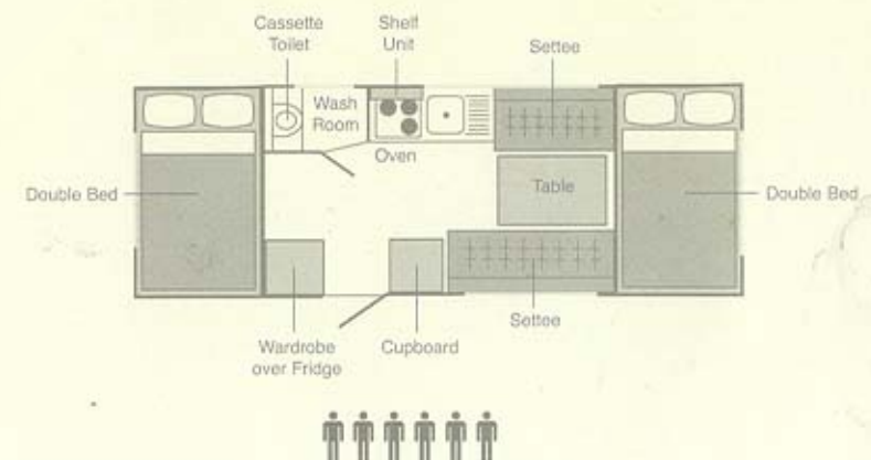
CAMPER WITH OPTIONAL AWNING
