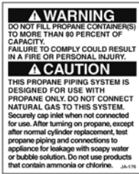
Fig. 7.4 “Do not fill to more than 80%” label
