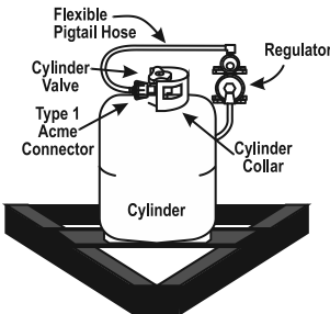
Fig. 7.5 Single cylinder
