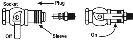
Fig. 10.2 Quick connect coupler
