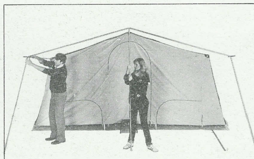
16. Add side cabin roof poles and legs.
