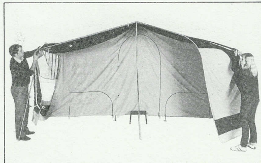
17. Pull forward extension canvas from main tent and locate short canopy poles through gussets.
