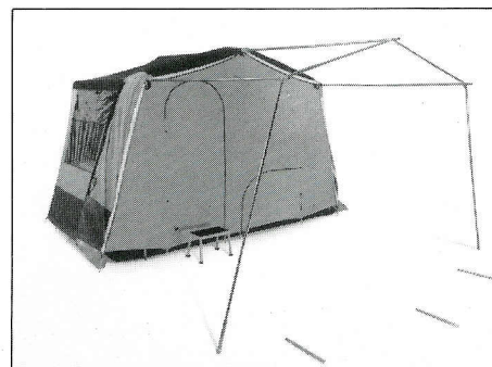
11 Hook roof support poles to main body frame and build up extension frame.
