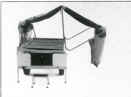
4 Swing over left hand support frame.
