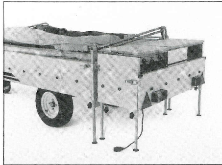
2 Drop the four kitchen support legs to within 1/2" off the ground, release the two protex fasteners. Disconnect the 7 pin plug before removing the kitchen from the slide support rails.
