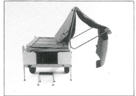
3 Swing over right hand cabin roof support frames.
