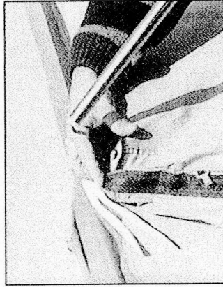
3. - Attach the three extension roof poles to the cabin frame. NOTE: The centre roof pole has a shorter hook.
