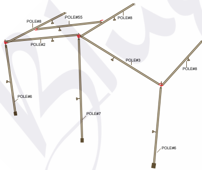
Camper Trailer Tent Outer Ridge 375 & Outer Ridge 475 awning poles
