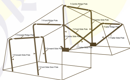
Camper Trailer Tent 7 tent poles
