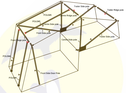
Camper Trailer tent 9, 9 Classic, 9 Deluxe tent poles
