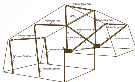
Camper Trailer Tent Outer Ridge 475 tent poles
