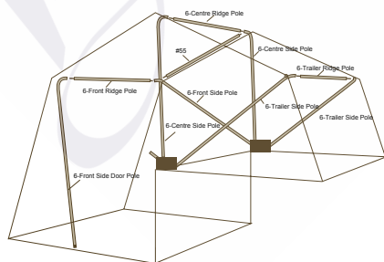
Camper Trailer Tent Outer Ridge 375 tent poles
