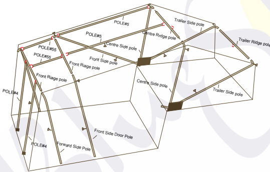
Camper Trailer Tent all 12 & 12 Twin tent poles
