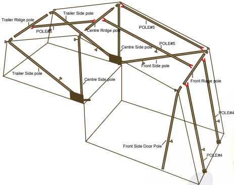
Camper Trailer Tent 8 & 8 Twin tent poles
