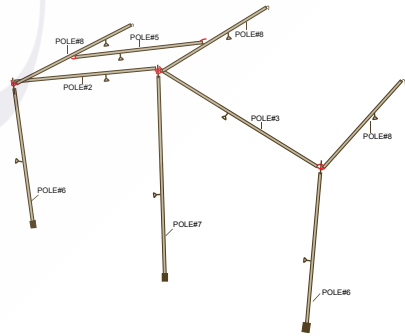
Camper Trailer Tent 8, 8 Twin & all 9 awning poles
