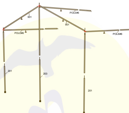
Camper Trailer Tent 6 & 7 awning poles
